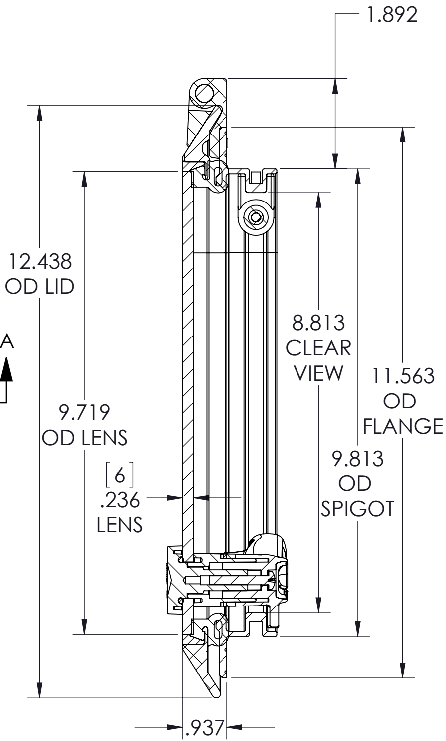
SECTION B-B
